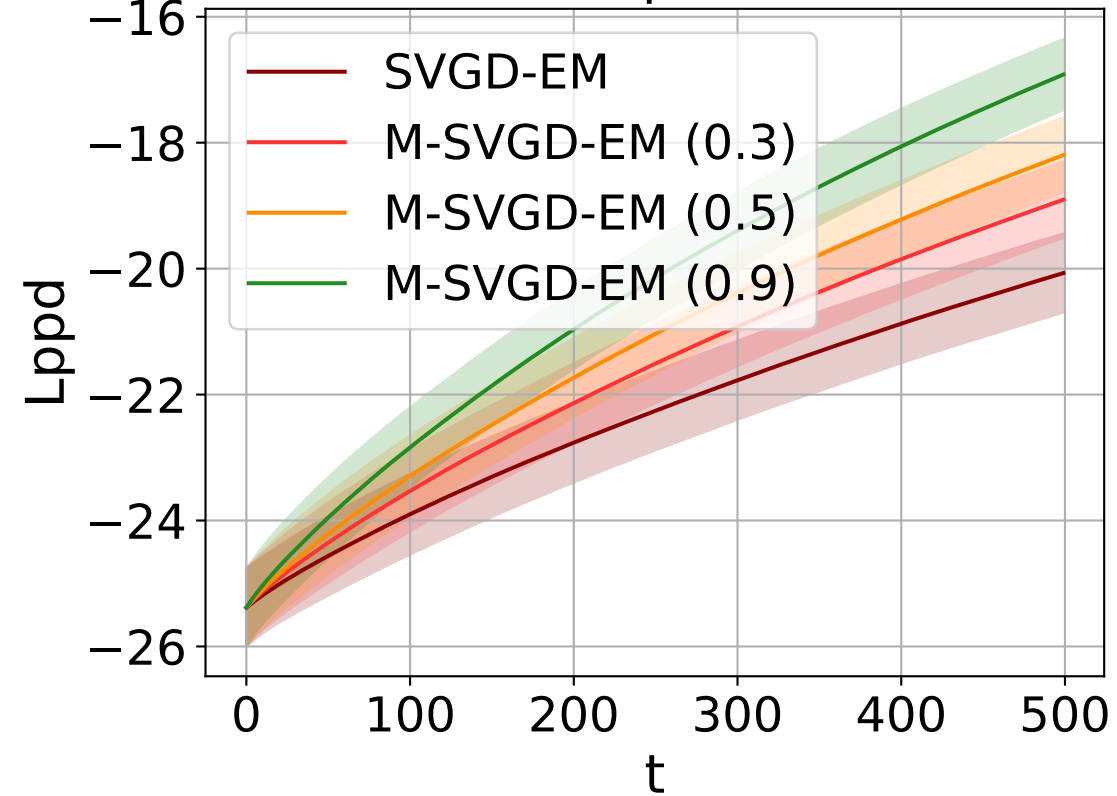
N = 20 particles
