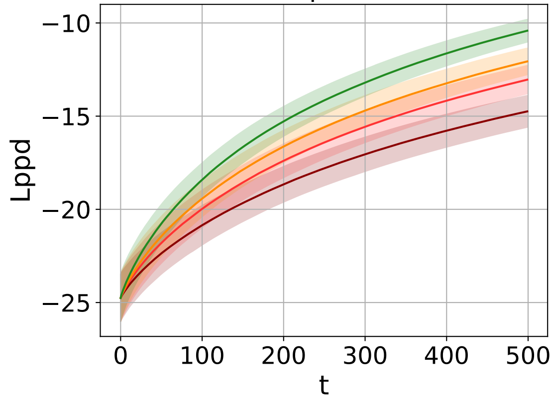
N = 5 particles
